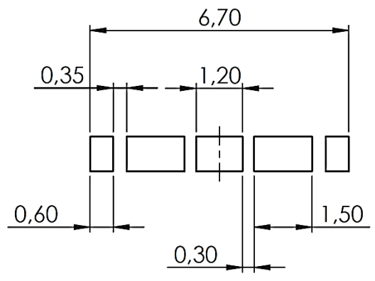
Detail B (8 : 1)
