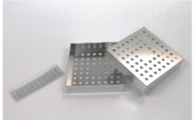
Picture only shows an example of a one-piece board level shield with clips
